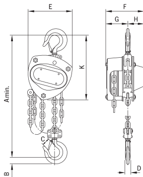
Model VSIII, 250 - 3000 kg, single fall
